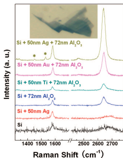
Figure 3. Raman spectra of graphene on different kinds of substrates. For original Si (without oxide layer) and Si/50 nm Ag substrates, the Raman spectra of few-layer (<5) graphenes instead of monolayer graphene were presented and taken at a laser power of about 10 mW and collection time of 1800 s and laser power of about 1 mW and collection time of 1200 s, respectively, since the monolayer graphene on these two substrates is nearly invisible and it is difficult to locate them for Raman measurements. For the other substrates, the Raman spectra were taken at a laser power of about 1 mW and a shorter collection time of 120 s. It reveals that the enhancement is different for different substrates, and the Raman signals of monolayer graphene are dramatically enhanced on the SMO substrates (Si/Ag/ \text{Al}_2\text{O}_3 and Si/Au/ \text{Al}_2\text{O}_3 ) compared with those on an IERS substrate of Si/ \text{Al}_2\text{O}_3 , or on a typical SERS substrate of Si/Ag and on an original Si wafer. Note that if the sandwiched metal layer, such as Ti, in a SMO substrate is not SERS-active, the Raman signals of graphene are not enhanced compared with the corresponding IERS substrate. The inset is the optical image of graphene on this Si/Ag/ \text{Al}_2\text{O}_3 substrate.
